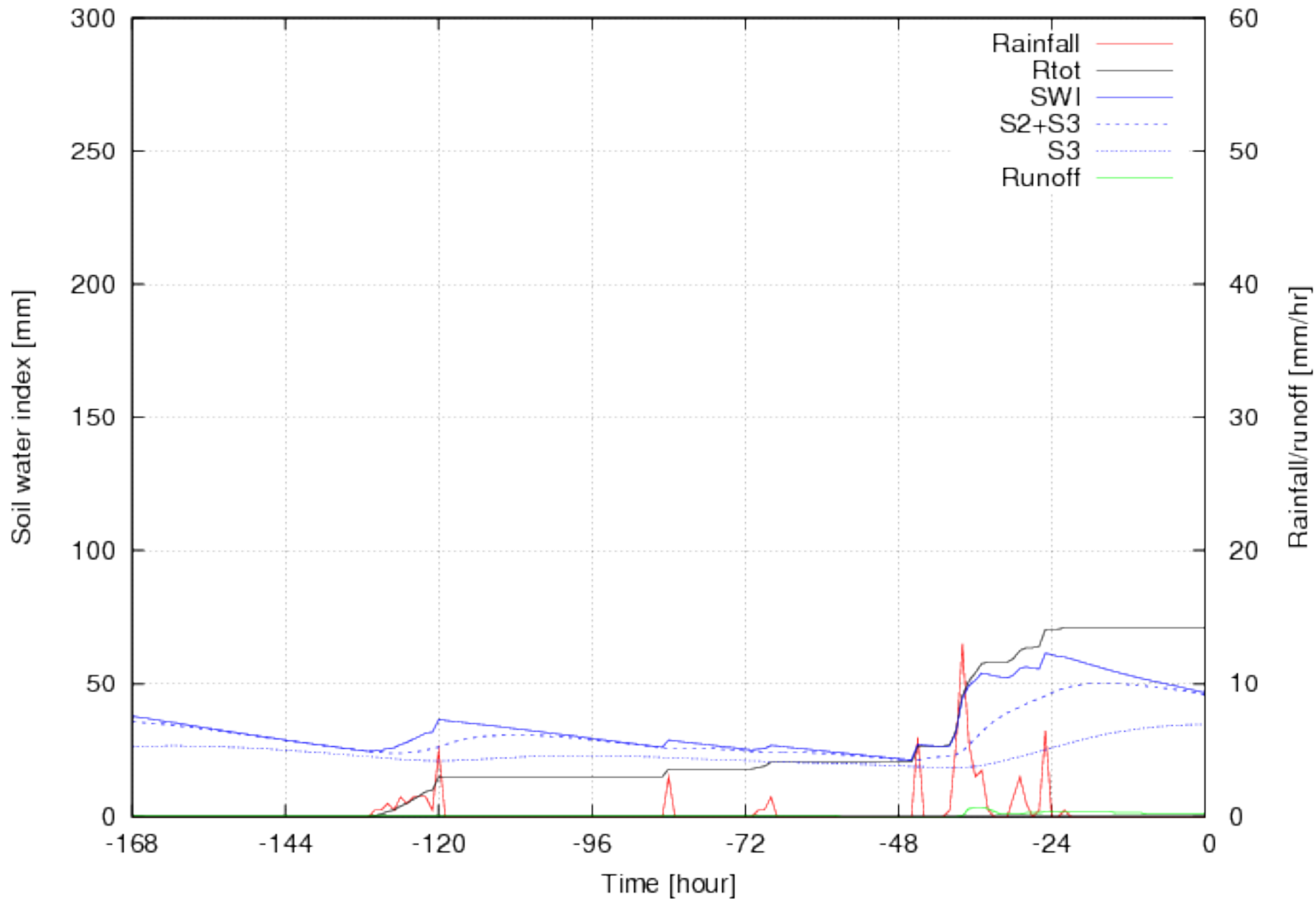
Rainfall & soil water index until 24:00, Mar. 24 at 44228
